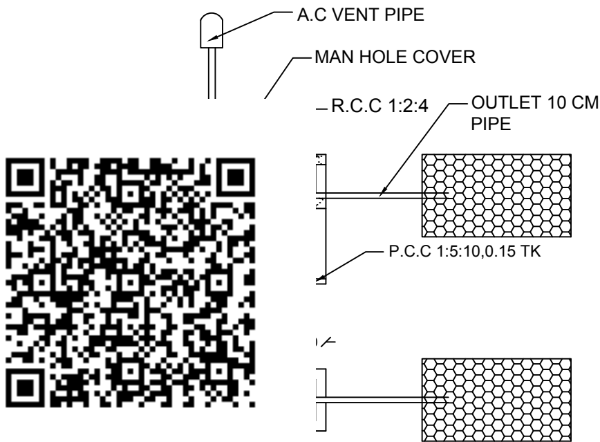
PLAN OF SEPTIC TANK & TRENCH
