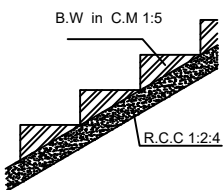
STAIRCASE
