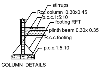
COLUMN DETAILS
