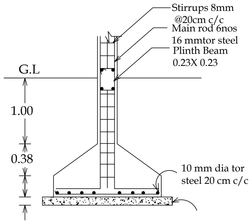
Details of coloumn footing
