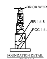
FOUNDATION DETAIL NOT TO SCALE
