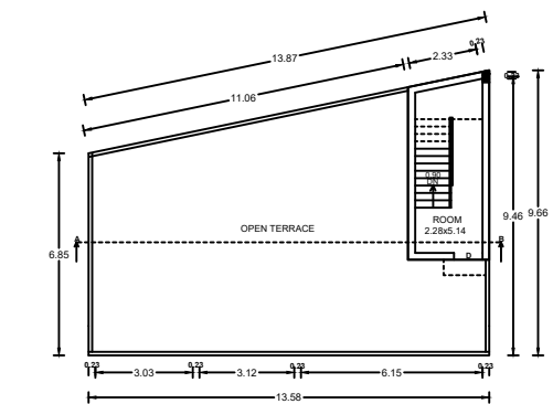
PROPOSED HEAD ROOM PLAN
