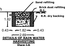
DETAILS OF RAIN WATER HARVESTING Dwg:1A
