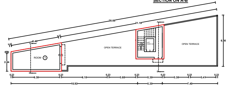
PROPOSED SECOND FLOOR PLAN
