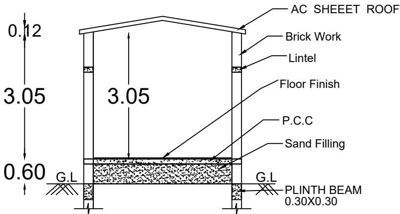
SECTION
