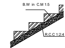
STAIRCASE
