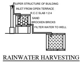
RAINWATER HARVESTING
