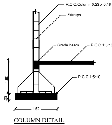
COLUMN DETAIL
