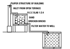
RAINWATER HARVESTING
