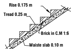
STAIR DETAILS
