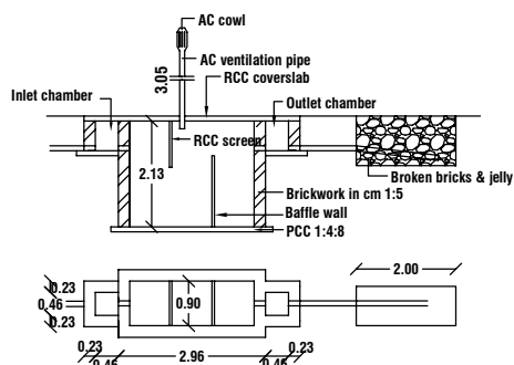
SEPTICTANK DETAILS
