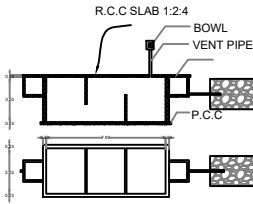
SEPTIC TANK AND TRENCH NTS
