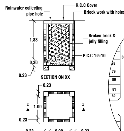
RAINWATER HARVEST WELL
