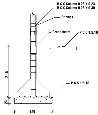
COLUMN DETAIL
