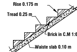
STAIR DETAILS
