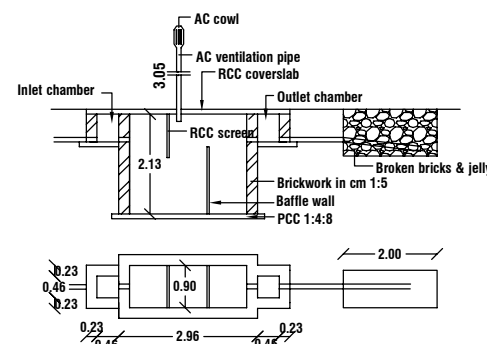
SEPTICTANK DETAILS
