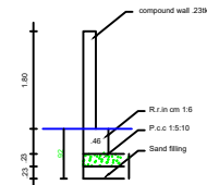
Compound Wall Detail SCALE (1:50)
