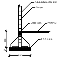
COLUMN DETAIL
