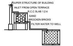
RAINWATER HARVESTING
