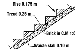
STAIR DETAILS
