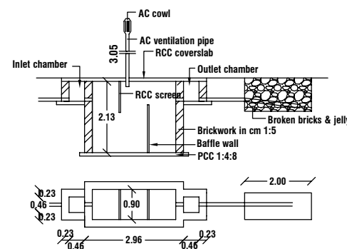
SEPTICTANK DETAILS
