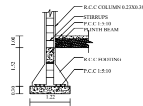
COLUMN DETAILS
