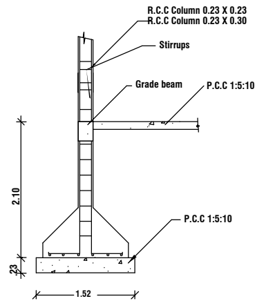
COLUMN DETAIL
