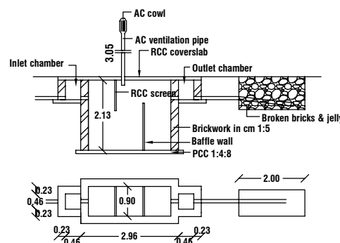
SEPTICTANK DETAILS
