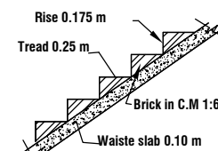
STAIR DETAILS
