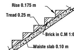
STAIR DETAILS
