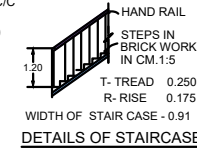
DETAILS OF STAIRCASE
