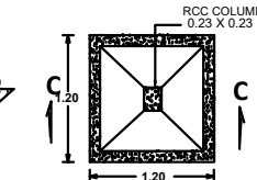
DETAILS OF COLUMN PLAN
