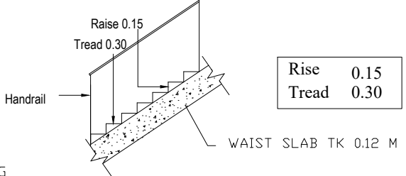
STAIRCASE DETAIL
