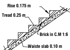
STAIR DETAILS
