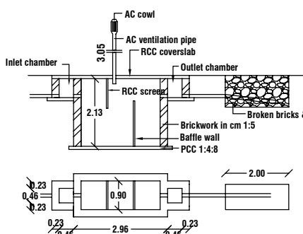
SEPTICTANK DETAILS
