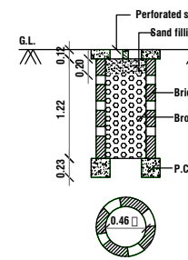
PERCOLATION PIT FOR 30 Sq. m. (Scale:- 1:50)
