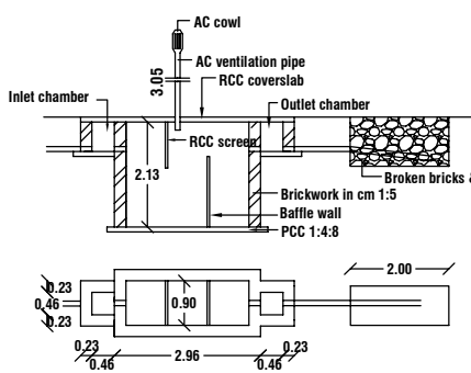
SEPTICTANK DETAILS
