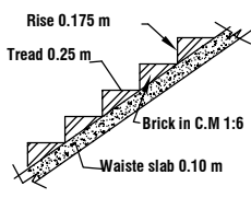
STAIR DETAILS
