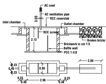
SEPTICTANK DETAILS
