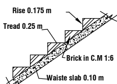
STAIR DETAILS
