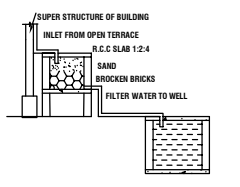
RAINWATER HARVESTING
