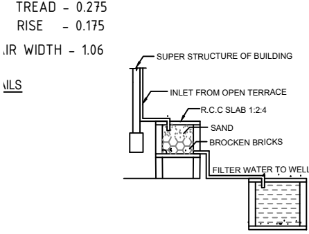
DETAILS OF FILTER BED & WELL
