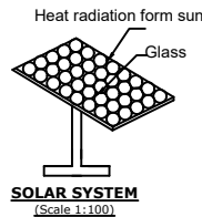
SOLAR SYSTEM
