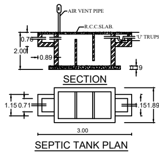
SEPTIC TANK PLAN
