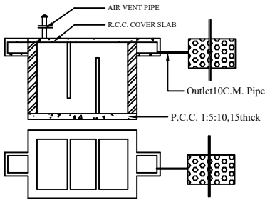
Exi. Septic Tank and Trench
