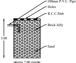
SECTION OF RAIN WATER COLLECTING TANK
