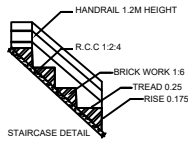
STAIRCASE DETAIL
