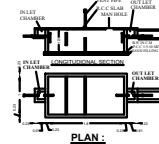
SEPTIC TANK
