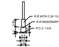
FOUNDATION
