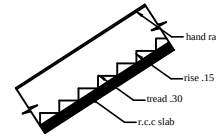
Stair
