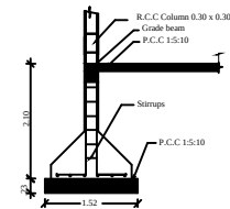
Column Detail
