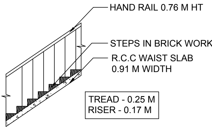
STEP DETAILS
