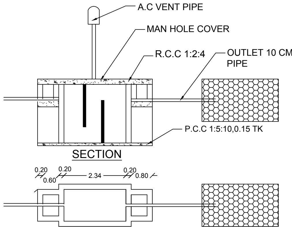
PLAN OF SEPTIC TANK & TRENCH
