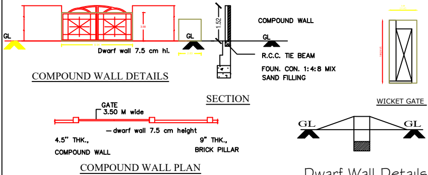
Dwarf Wall Details
