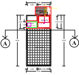
PRO. FIRST FLOOR PLAN.
