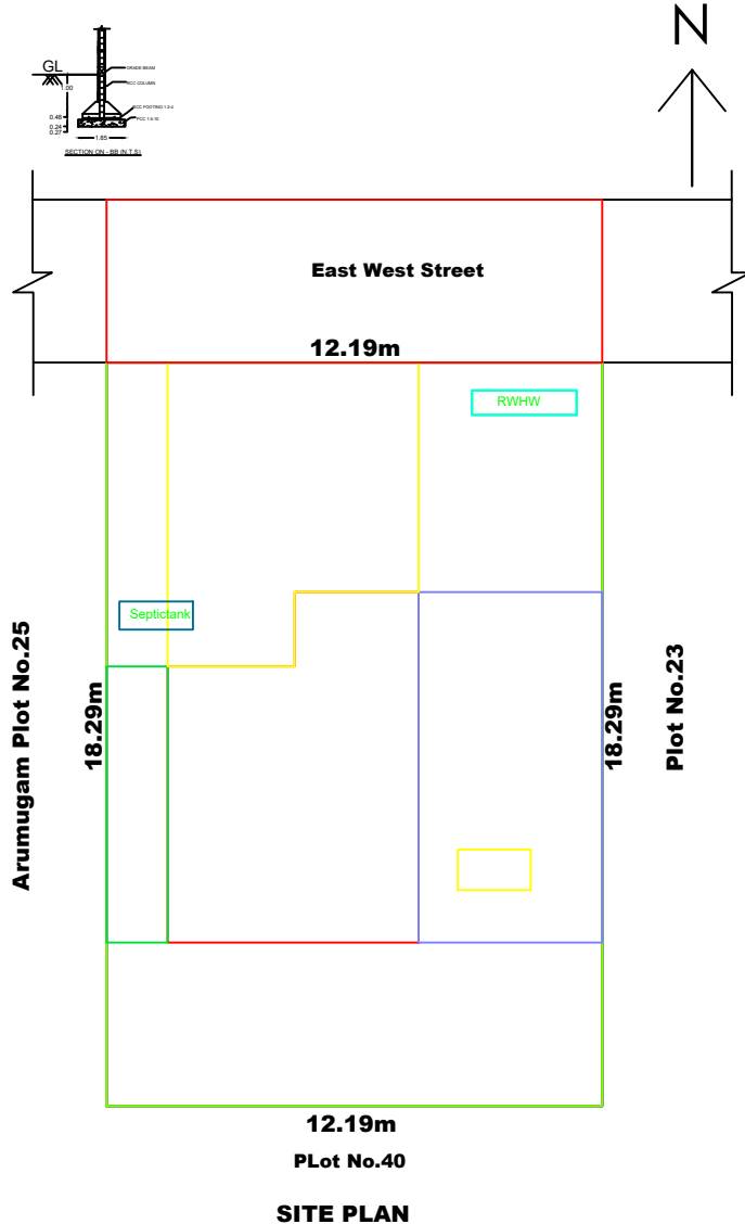
SITE PLAN
