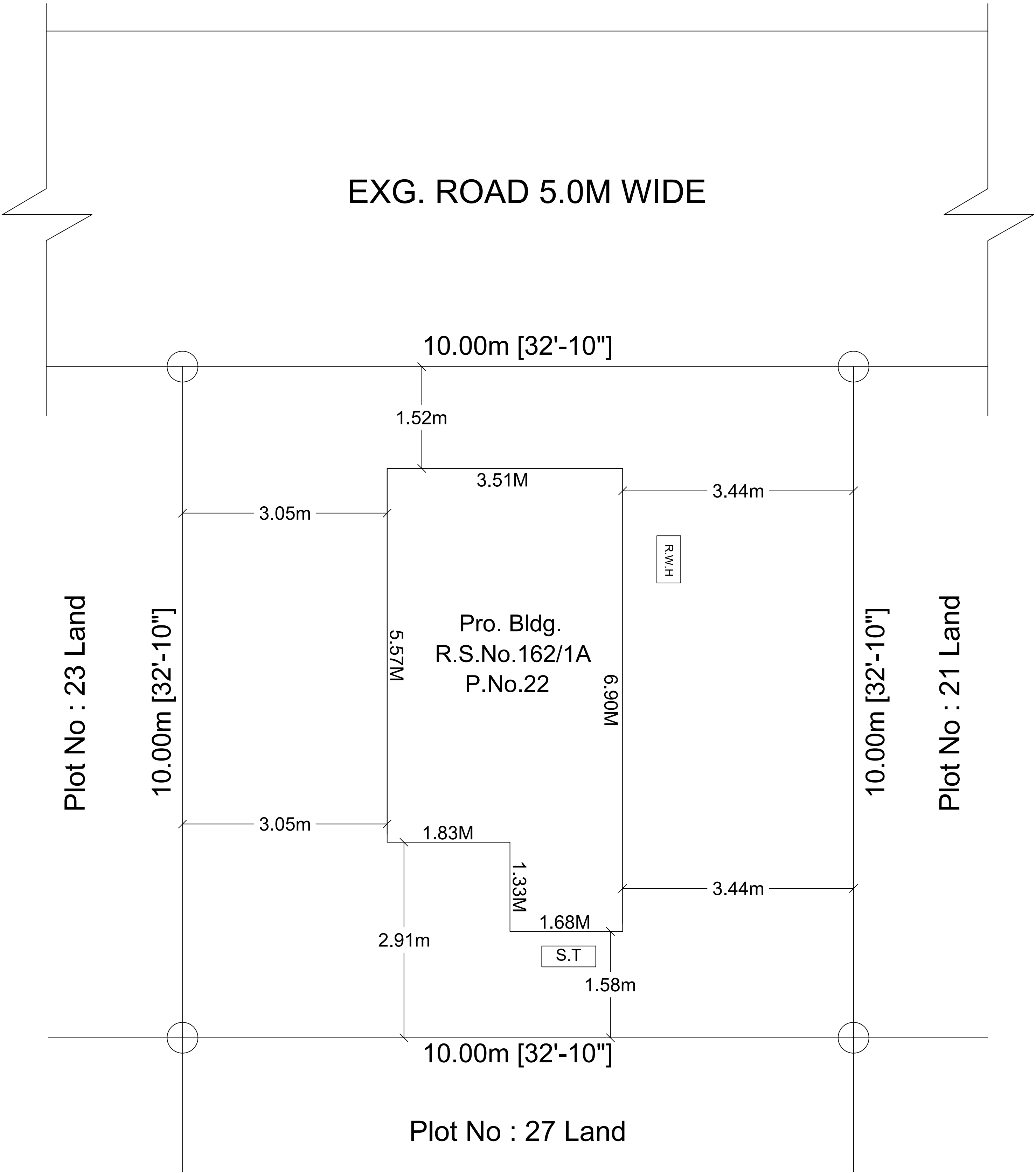
SITE PLAN
