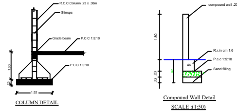
COLUMN DETAIL
