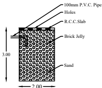
SECTION OF RAIN WATER COLLECTING TANK
