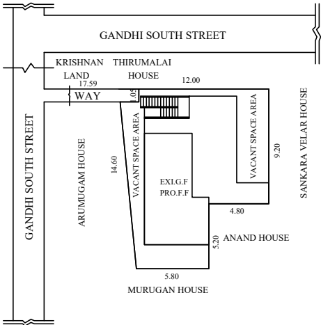
SITE PLAN
