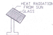
SOLAR SYSTEM
