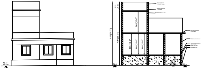
SECTION AB
