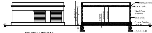
SECTION ON AA
