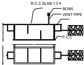
SEPTIC TANK AND TRENCH
