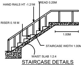
STAIRCASE DETAILS
