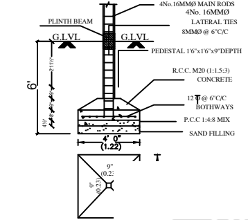
FOUNDATION
