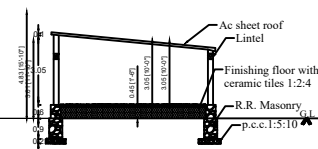
SECTION AB
