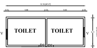
GROUND FLOOR PLAN-B
