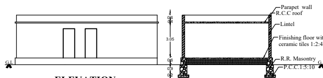
SECTION AB
