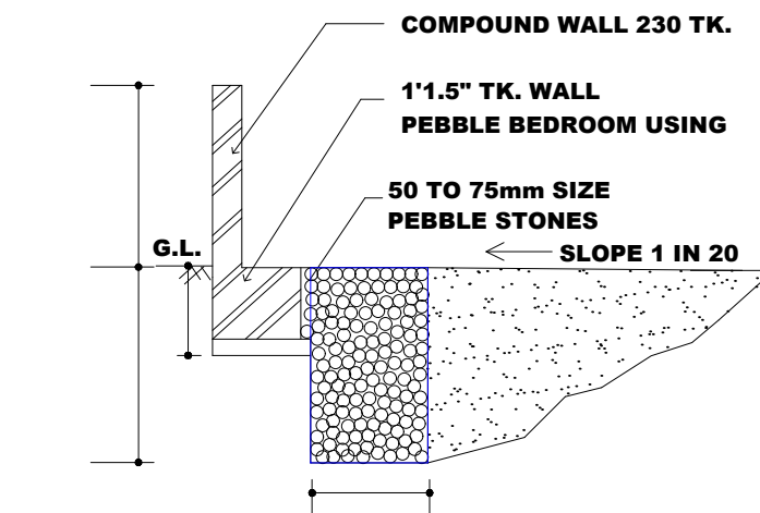
RAIN WATER COLLECTION TRENCH
