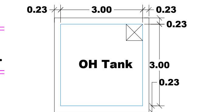
WATER_TANK_CAPACITY_L=13500LTRS
