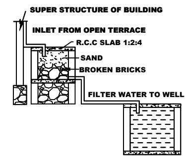
RAINWATER HARVESTING
