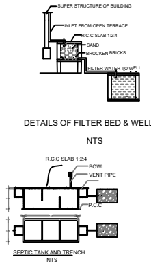
SEPTIC TANK AND TRENCH
