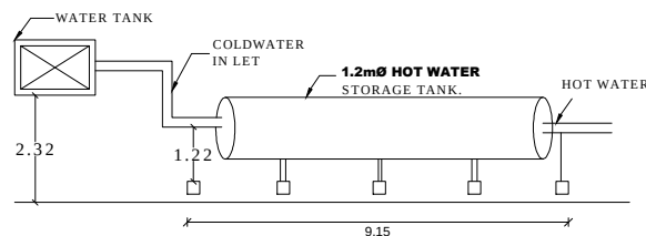
SOLAR WATER HEATING SWHS DETAIL
