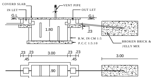
PLAN & SECTION OF SEPTIC TANK & TRENCH
