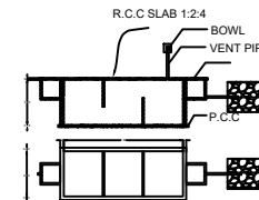
SEPTIC TANK AND TRENCH NTS
