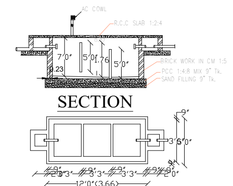
SECTION PLAN SEPTIC TANK DETAILS
