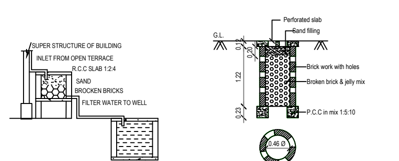
RAINWATER HARVESTING PERCOLATION PIT FOR 30 Sq.m. (Scale:- 1:50)
