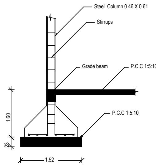
COLUMN DETAIL
