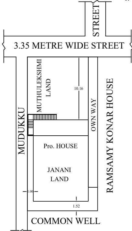
SITE PLAN
