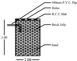
SECTION OF RAIN WATER COLLECTING TANK
