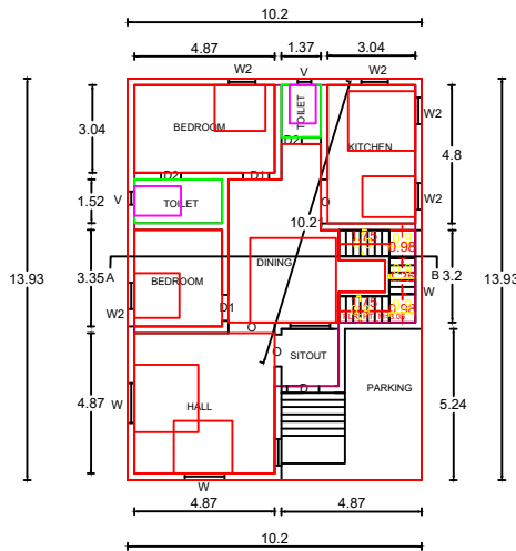
GROND FLOOR PLAN
