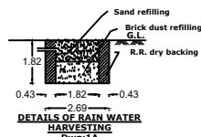
DETAILS OF RAIN WATER HARVESTING Dwg:1A
