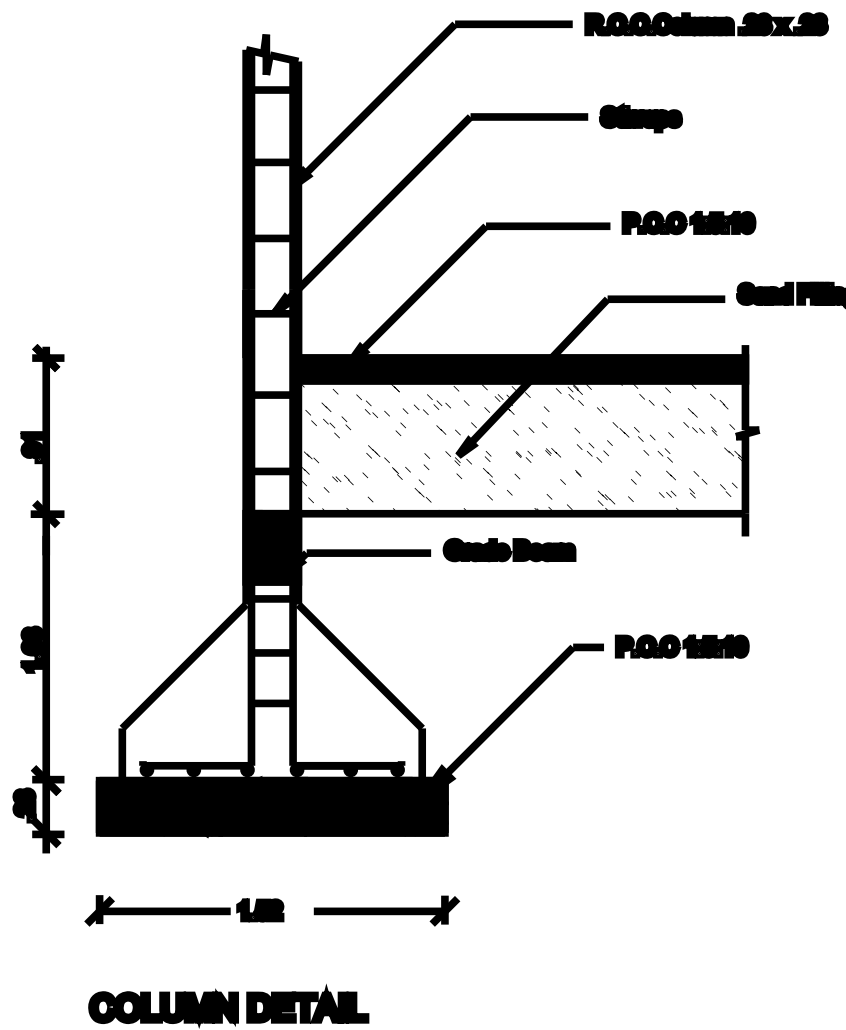
COLUMN DETAIL
