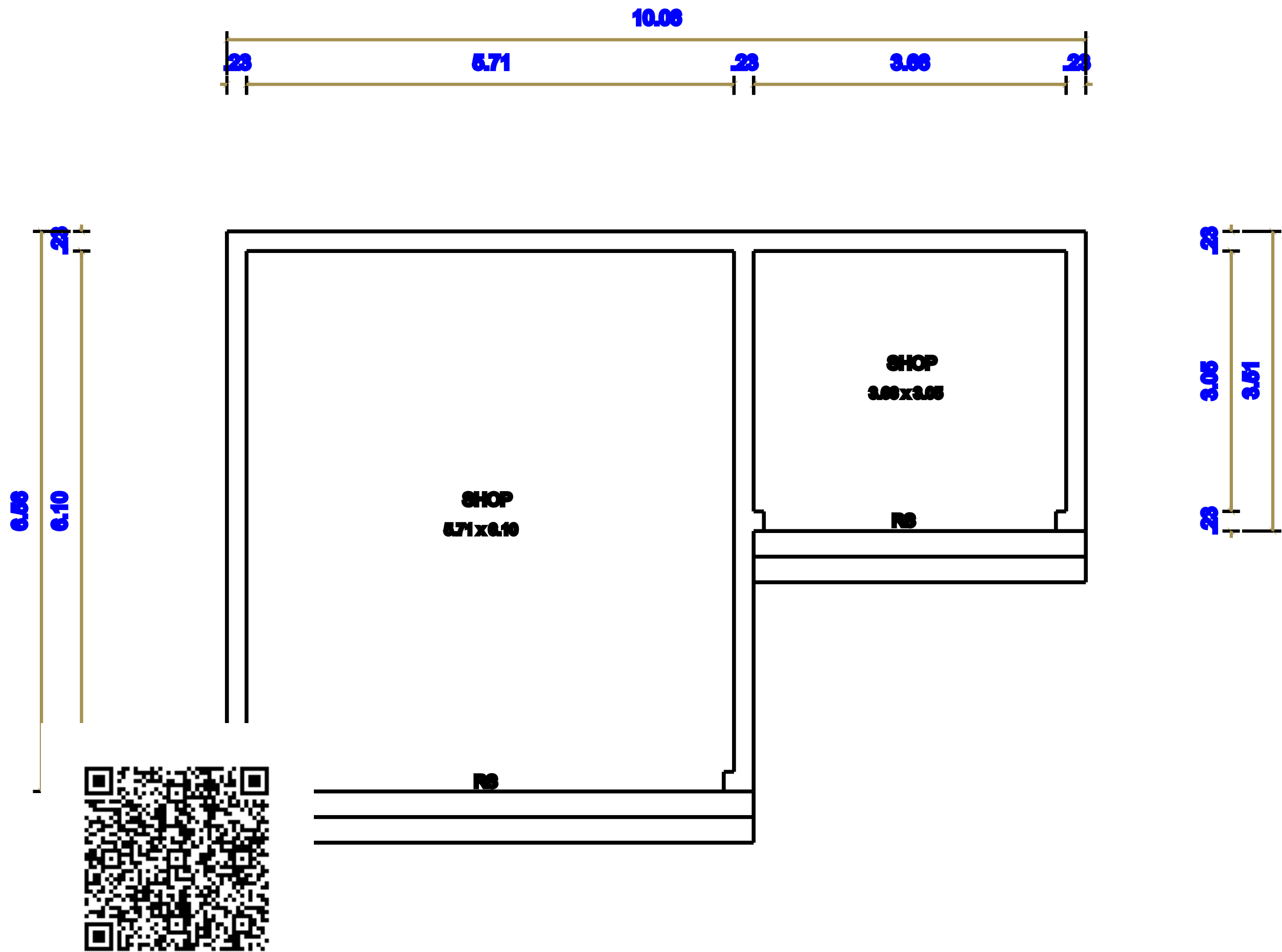
PLAN
