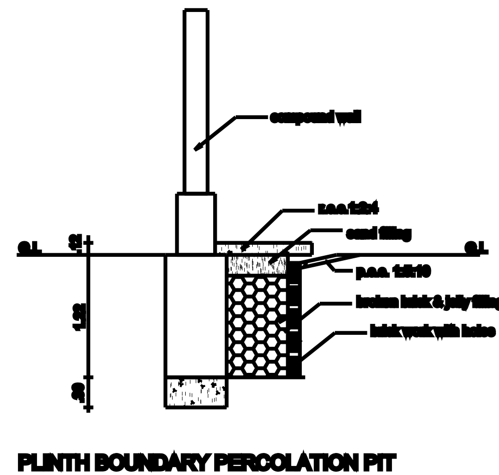
PLINTH BOUNDARY PERCOLATION PIT
