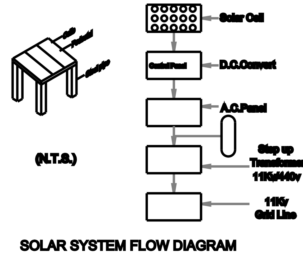
SOLAR SYSTEM FLOW DIAGRAM
