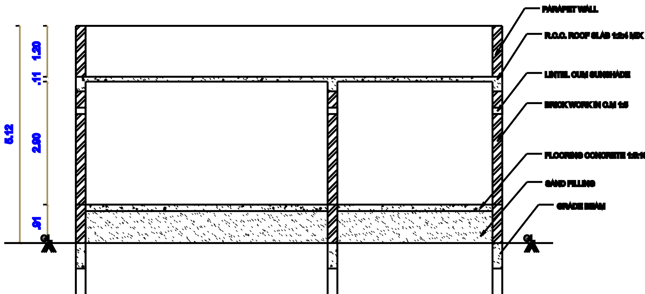
SECTION-AA
