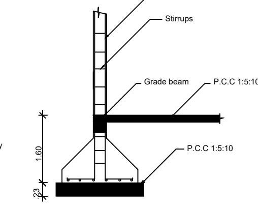
COLUMN DETAIL
