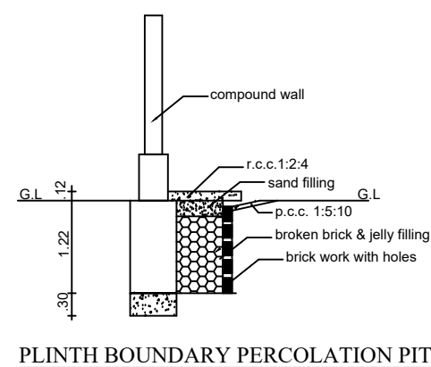
PLINTH BOUNDARY PERCOLATION PIT
