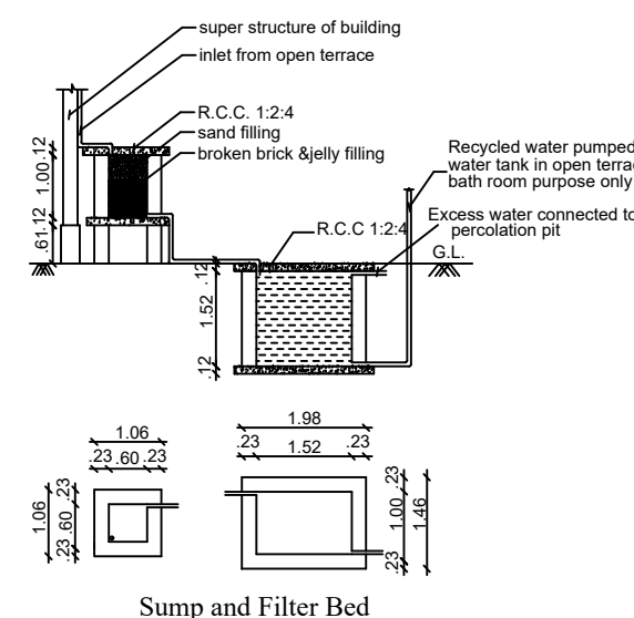
Sump and Filter Bed
