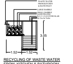
RECYCLING OF WASTE WATER FROM KITCHEN & BATHROOM
